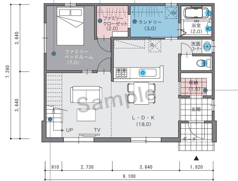
< Main Floor >
